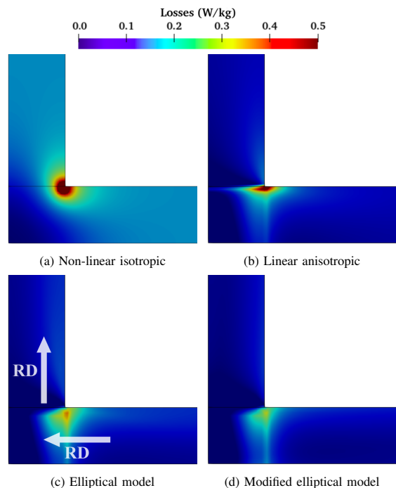
Fig. 2. Specific iron losses (W/kg) of the upper laminations per model.
