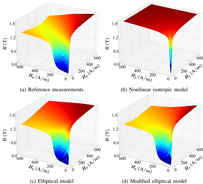
Fig. 1. Induction level as a function of the field components.
