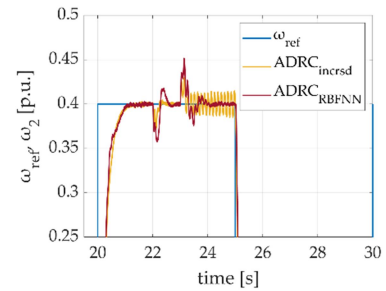
Fig. 4. The load speed transients for changed time constant value including modified control structures (zoom).
