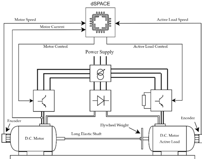
Fig. 2. Schematic diagram of experimental setup with a two-mass system.
