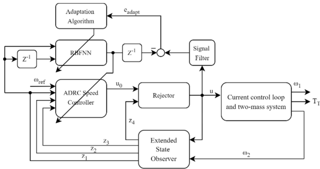
Fig. 1. The proposed ADRC structure with neural parameters adjustment.
