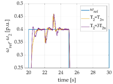
Fig. 3. Results (speed transients) of ADRC algorithm (applied for a drive with elastic connection) achieved under different values of the load machine time constant.
