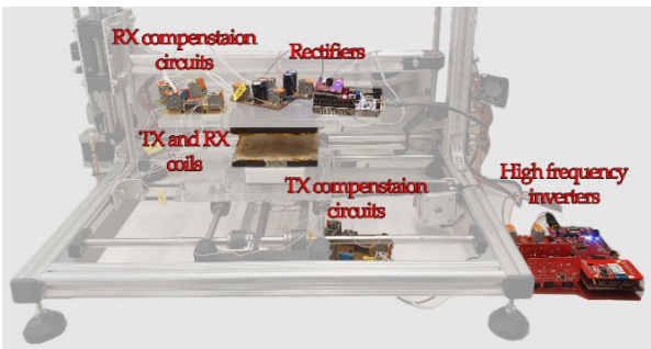
Fig.2. Multi-coil experimental platform.
