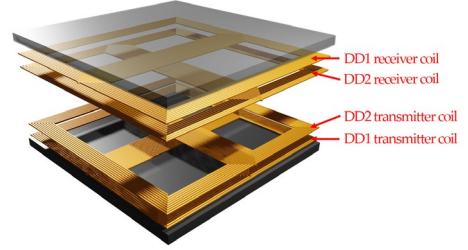
Fig.1. Basic double DD transmitter and receiver coil structure
