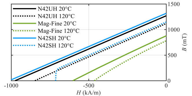
Figure 1: Demagnetization curves for evaluated PM materials at 20°C and 120°C.
